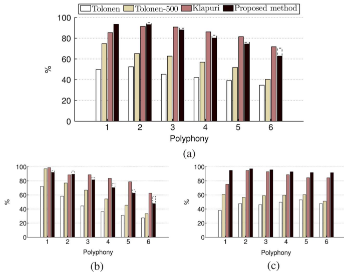
Fig. 7. Multipitch estimation results with unknown polyphony: for each algorithm, the F-measure, the precision and the recall are rendered as a function of the true polyphony. For the proposed method, the performance on the training set is plotted using a dashed line. (a) F-measure. (b) Recall. (c) Precision.
