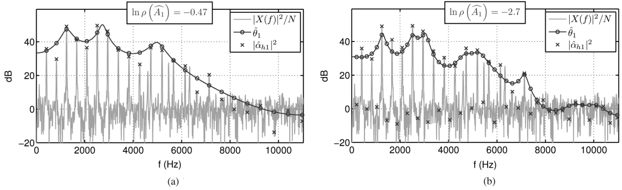
Fig. 2. Estimation of spectral envelopes: the AR estimation performs a better fitting of the amplitudes for the correct model (left) than for the sub-octave model (right). (a) True note: A\flat_4 . Selected model: A\flat_4 . (b) True note: A\flat_4 . Selected model: A\flat_3 .
