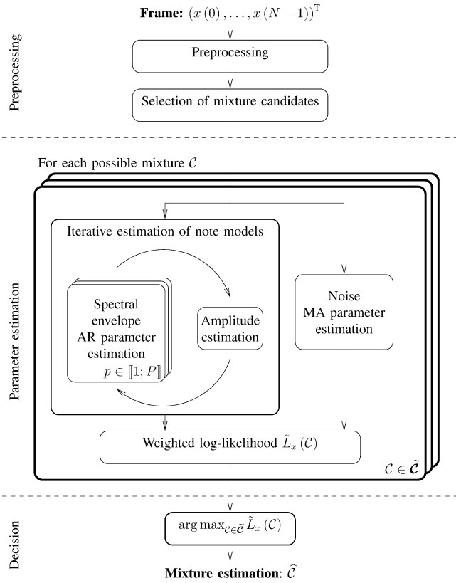
Fig. 1. Multipitch estimation block diagram.
