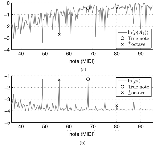
Fig. 6. \ln \rho(\widehat{A}_1) (top) and \ln \rho_b(\widehat{B}) (bottom) as a function of a single-note model (true note: A\flat_4 ). (a) \ln \rho(\widehat{A}_p) . (b) \ln \rho_b(\widehat{B}) .
