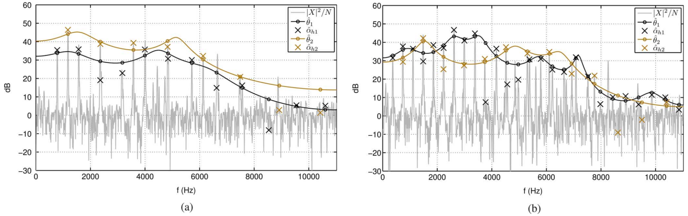
Fig. 4. Iterative estimation of amplitudes \hat{\alpha}_p and spectral envelopes \hat{\theta}_p : example of a fifth [Fig. 4(a)] and of an octave [Fig. 4(b)]. (a) True notes: G_5 + D_6 . Selected model: G_5 + D_6 . (b) True notes: F\#_4 + F\#_5 . Selected model: F\#_4 + F\#_5 .
