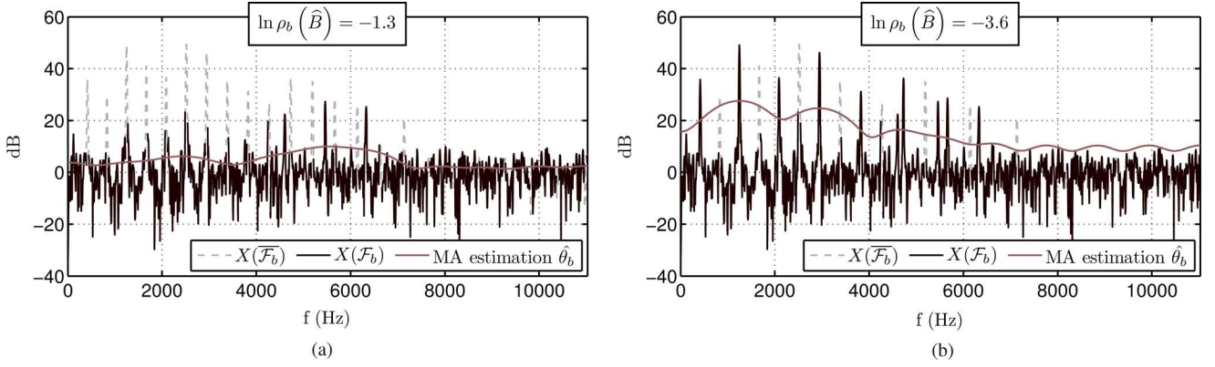
Fig. 5. Noise parameter estimation when selecting the true model (left) and the octave model (right). \overline{\mathcal{F}_b} denotes the complement of \mathcal{F}_b . (a) True note: Eb_4 . Selected model: Eb_4 . (b) True note: Eb_4 . Selected model: Eb_5 .
