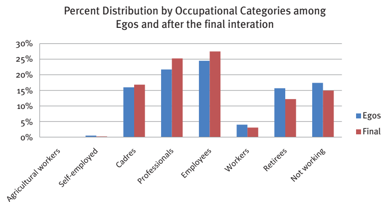
Figure 1.10 Percentage distribution of Occupational categories.
