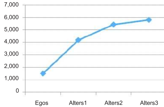
Figure 1.5 Cumulative number in our population who received the advisory in three iterations.
