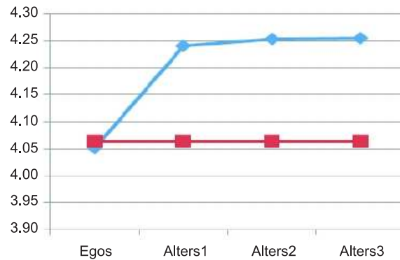
Figure 1.9 Blue: average food risk knowledge of those who have the information. Red: Average food risk knowledge of overall population.
