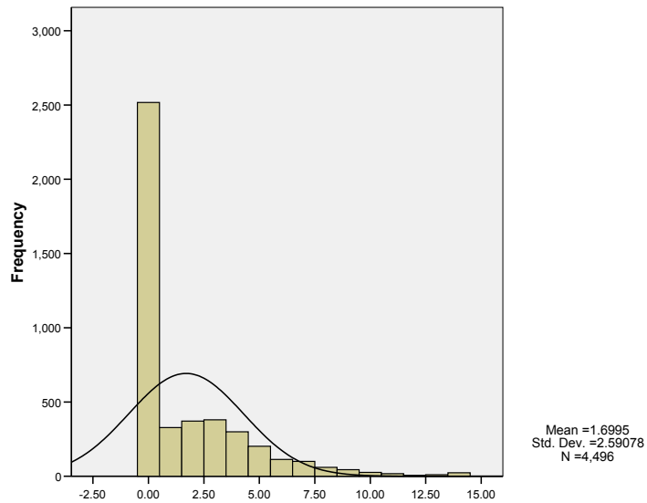
Figure 1.1 The distribution of the number of transmissions reported by Egos.
