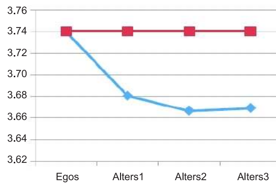
Figure 1.8 Blue: average education of those who have the information. Red: Average education of overall population.
