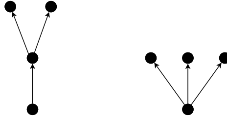
Figure 1.2 An illustration of the difference between \mu_h and \xi measures, in which edges represent information transmissions between vertices. For the graph on the left there is one original sender, two senders and three transmissions and receivers, hence \mu_h = 3 and \xi = 3/2 . For the one on the right there is only one sender and \mu_h = 3 and \xi = 3 .
