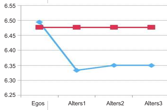
Figure 1.7 Blue: average age of those who have the information. Red: Average age of overall population.
