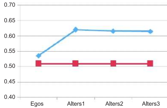
Figure 1.6 Blue: proportion of those who have the information. Red: over-all population proportion.
