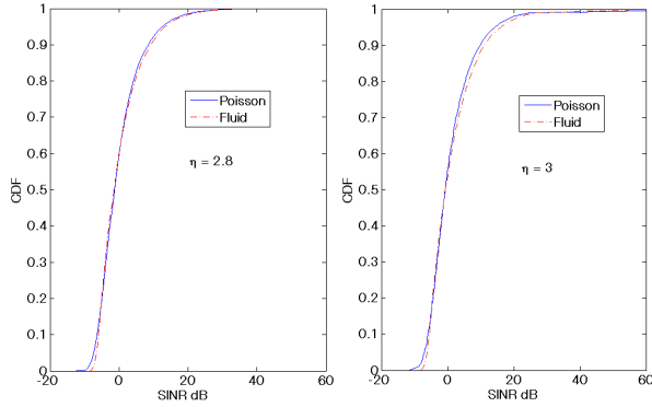
Fig. 5. CDF of the fitted SINR with \eta = 2.8 (left) and \eta = 3 (right), for a Poisson model network and a Fluid model network.
