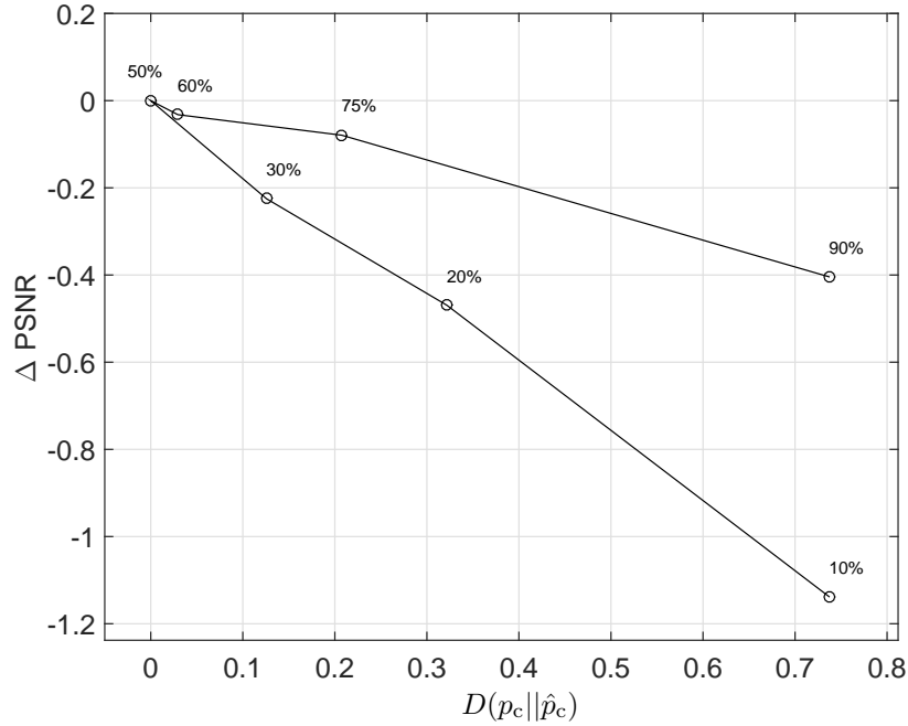
Figure 15 Graph of the PSNR losses of the proposed technique vs. the relative entropy of the estimated preference distribution with respect to perfect estimation p_c = 50\% . M = 2 and \varepsilon = 10\% .
