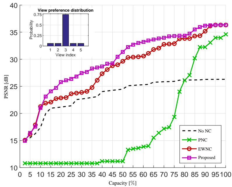
(b) M = 2 \varepsilon = 30\% p_c = 75\%
