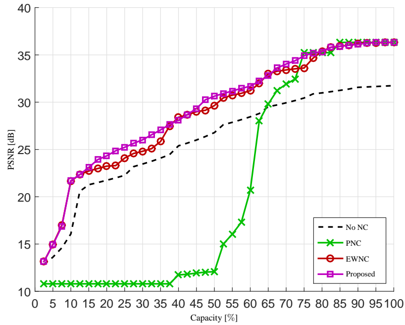
(a) M = 2 Gilbert – Elliot model p_c = 50\%
