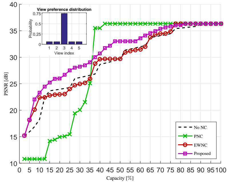
(b) M = 4 \varepsilon = 30\% p_c = 75\%
