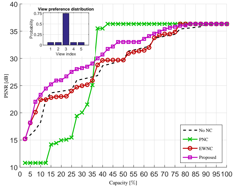
(a) M = 4 \varepsilon = 10\% p_c = 75\%
