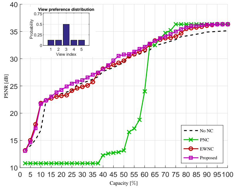
(a) M = 2 \varepsilon = 10\% p_c = 50\%
