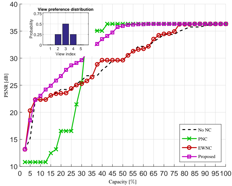
(a) M = 4 \varepsilon = 10\% p_c = 50\%
