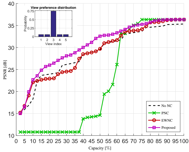
(a) M = 2 \varepsilon = 10\% p_c = 75\%
