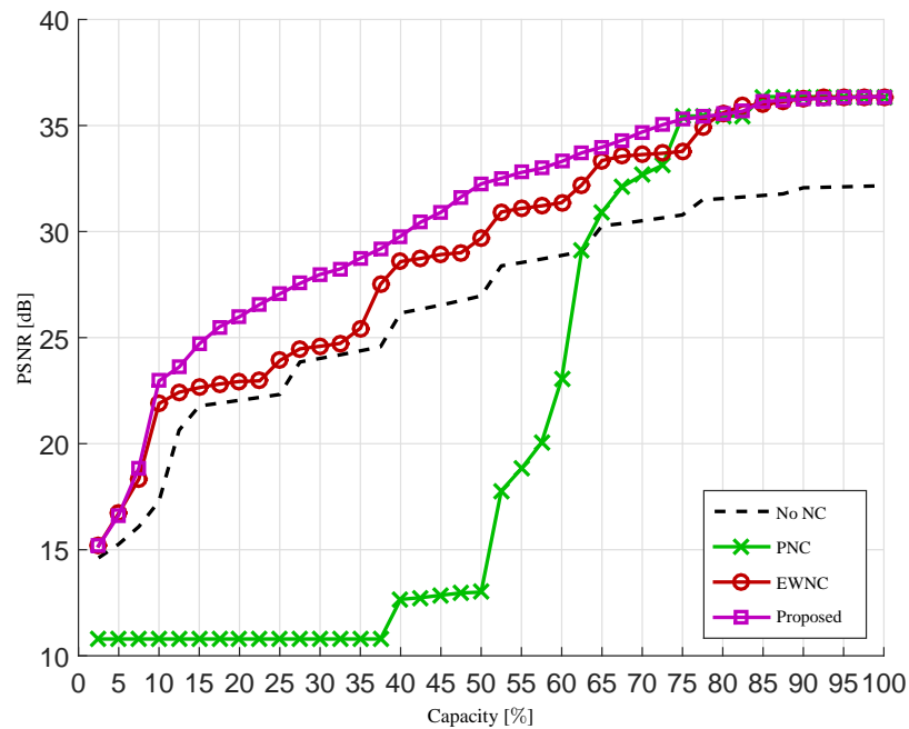
(b) M = 2 Gilbert – Elliot model p_c = 75\%
