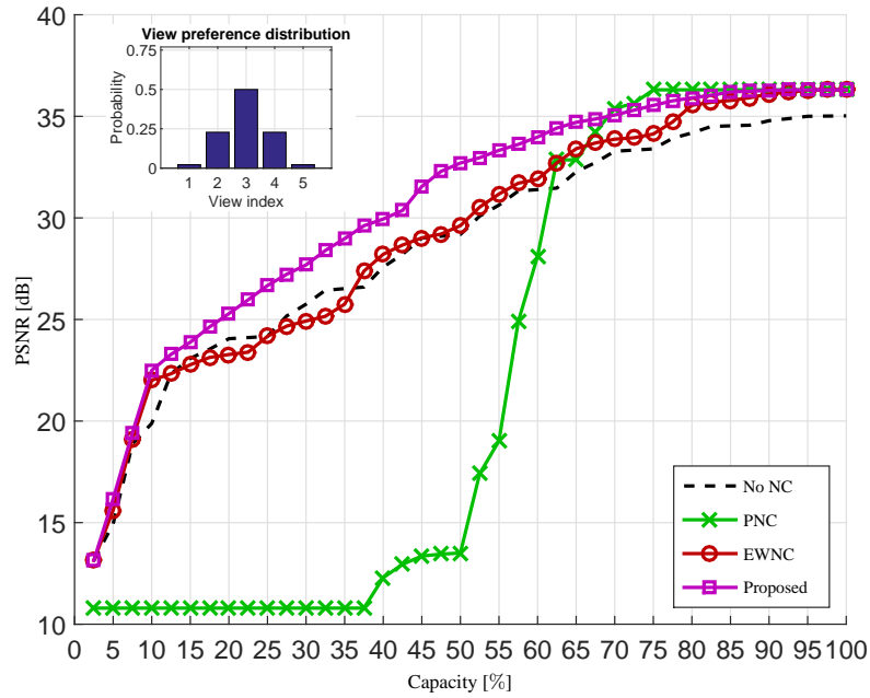
(a) M = 2 \varepsilon = 10\% p_c = 50\%
