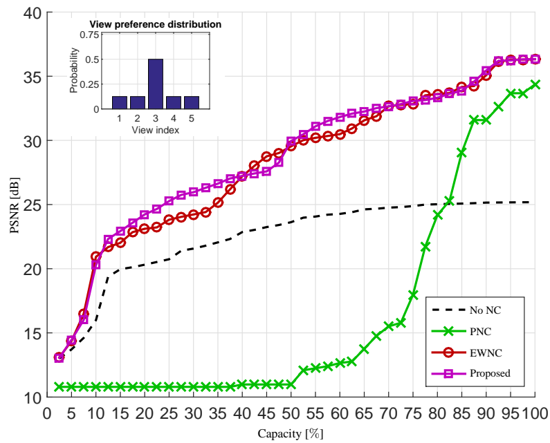
(b) M = 2 \varepsilon = 30\% p_c = 50\%
