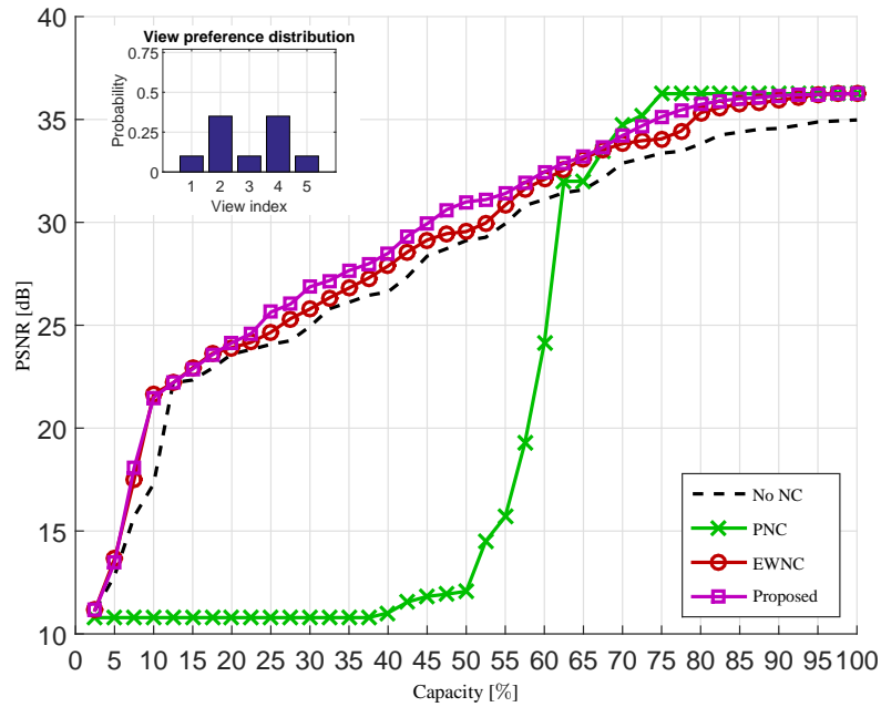
(b) M = 2 \varepsilon = 30\% p_c = 35\%
