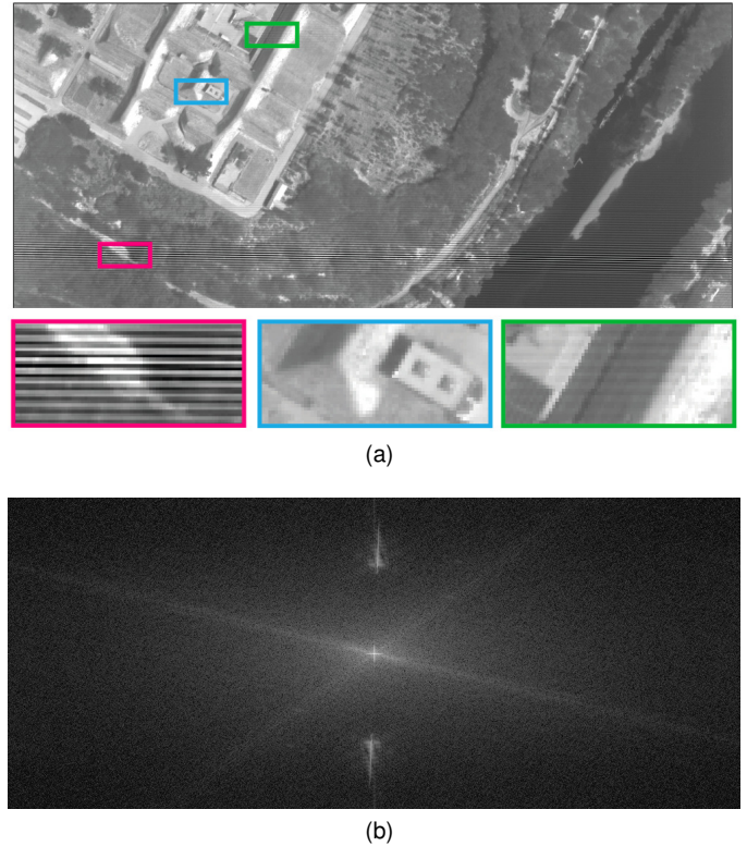
Fig. 1. On top, an image obtained with Sietelets. Subimages are magnified to show the interference fringes overlaid on the scene. In red, an area with highly contrasted fringes. In blue, an area with blurred fringes. In green, an area with slightly contrasted fringes. The area with high contrast fringes is limited to the area around the zero optical path difference, due to the broadband observed spectra. Nonetheless, fringes are actually present over the whole image. Image (b) shows the Fourier spectrum of picture (a). The frequencies of the fringes are clearly seen as two very bright vertical lines. These frequencies constitute an area we call \Omega_0 .
