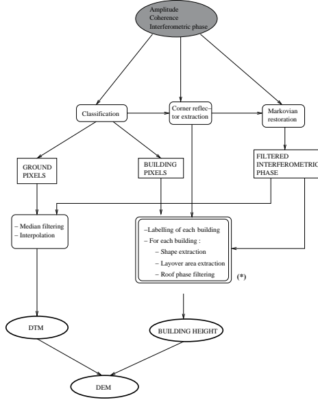
Figure 1: Graph of the global approach for DEM computing. The part (*) is detailed in this article.
