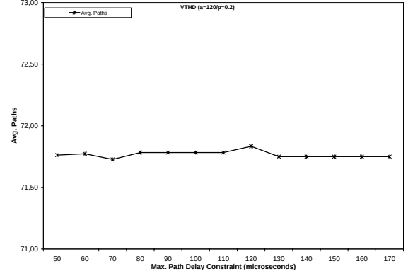
(b) VTHD, a = 120
