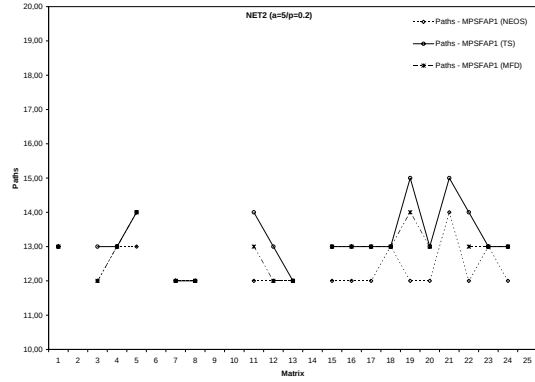
(b) Paths, a = 5
