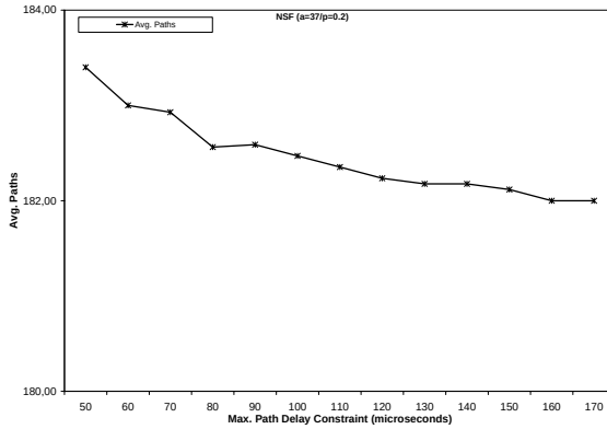
(a) NSF, a = 37
