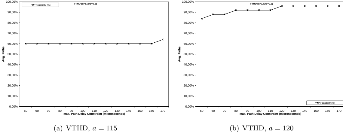
Figure 6.12: Feasibility Rate for VTHD Network Topologies Using MFD Algorithm, as a Function of Delay Constraint
