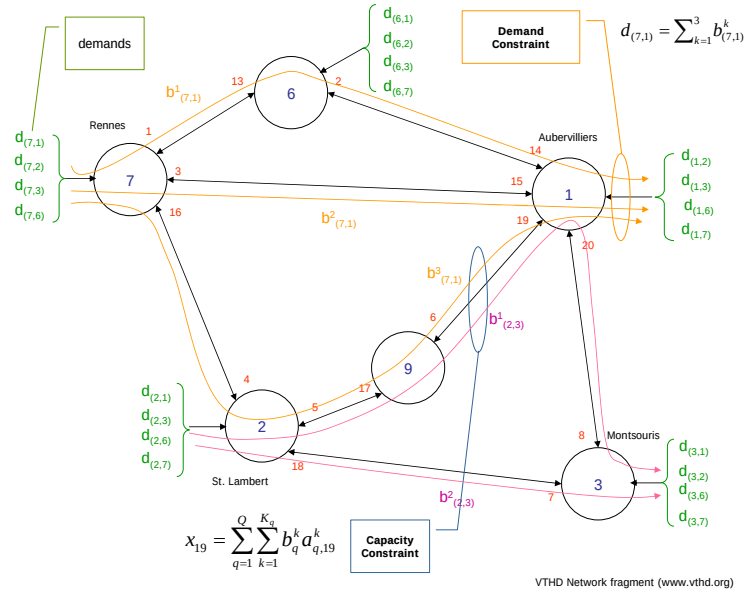
Figure 4.1: Path Flows: Relationship to Demands and Link Capacities
