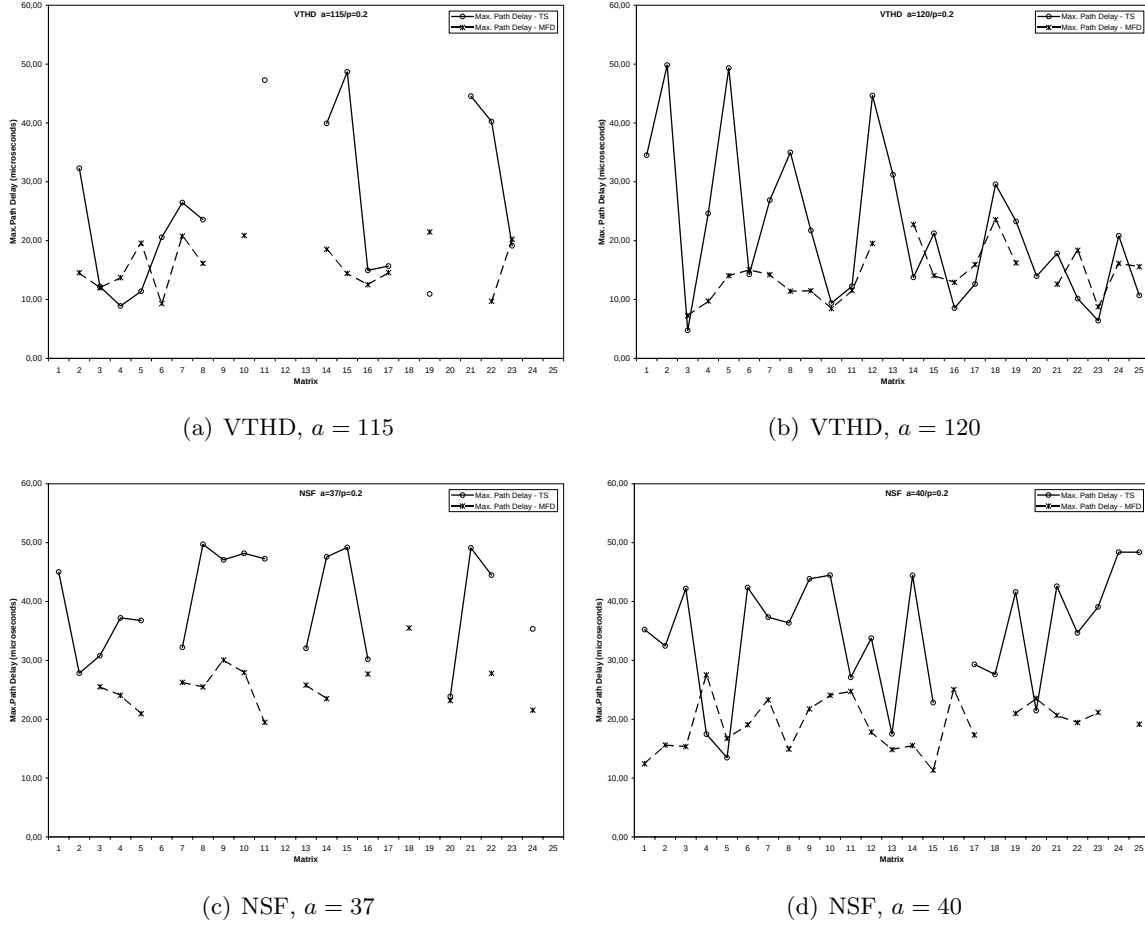
Figure 6.5: Maximum Path Delay in Layouts Obtained from MPSFAP1 for VTTHD and NSF Network Topologies using TS and MFD Algorithms
