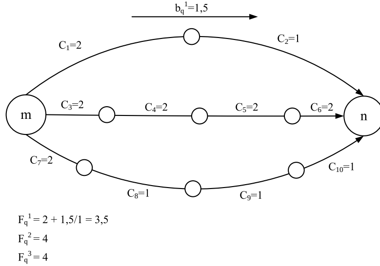
Figure 5.4: MFD Algorithm Example: Overloaded Path is Still the Shortest Path
