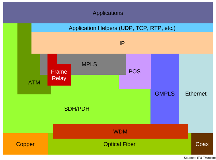
Figure 2.3: NGN Protocol Structure
