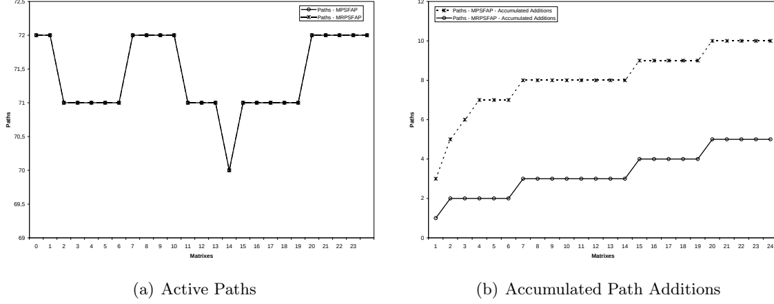
Figure 8.6: Active paths and accumulated path additions for MPSFAP1 and MRPSFAP on VTHD for demand matrix series M_1^{VTHD} using MFD and MFD-R heuristics
