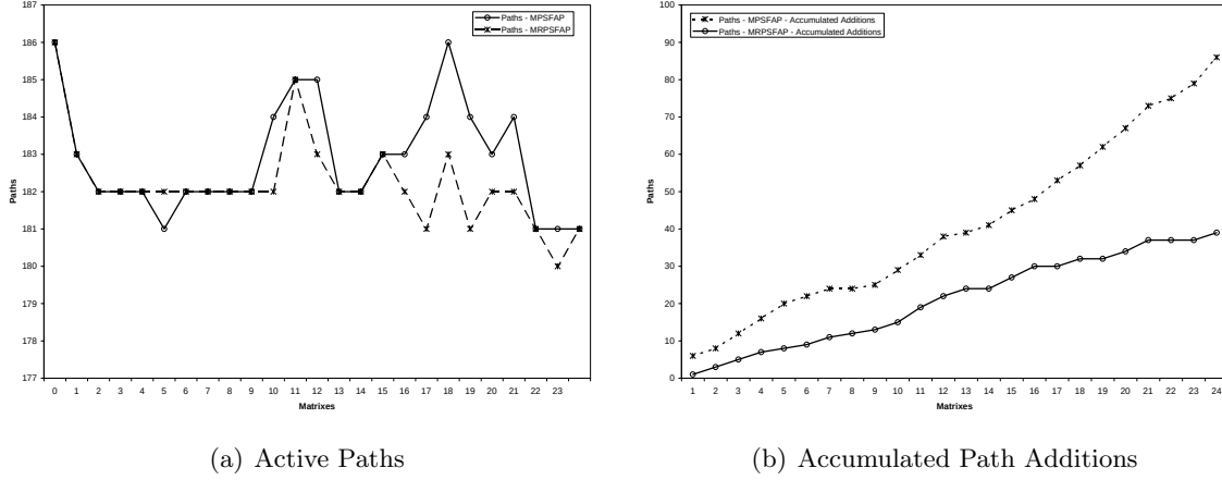
Figure 8.10: Active paths and accumulated path additions for MPSFAP1 and MRPSFAP on NSF for demand matrix series M_1^{NSF} using MFD and MFD-R heuristics
