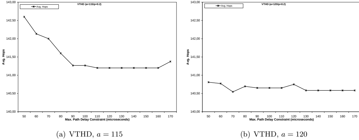
Figure 6.8: Average Quantity of Hops for VTHD Network Topologies Using MFD Algorithm, as a Function of Delay Constraint
