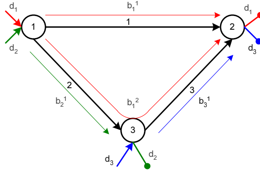
Figure 4.2: Example on the importance of avoiding path-delay constraints on unused paths
