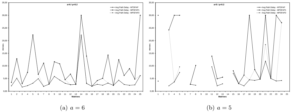
Figure 4.7: Maximum End-to-end Path Delay for NET2
