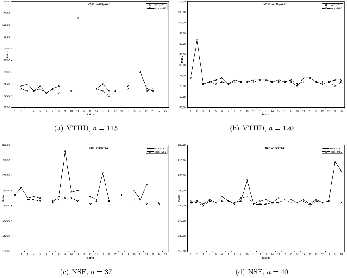
Figure 6.4: Used Paths for Layouts Obtained from MPSFAP1 for VTTHD and NSF Network Topologies using TS and MFD Algorithms
