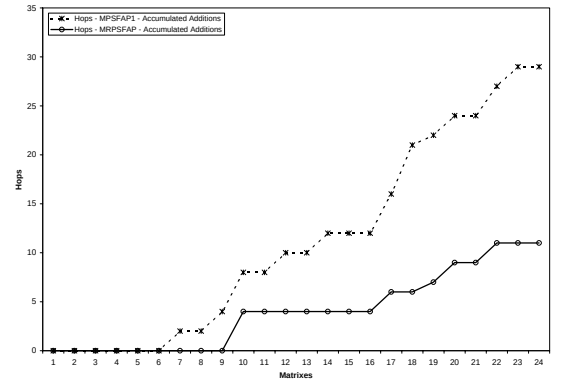
(b) Accumulated hops additions, a = 5, p = 0.2, p_v = 0.4
