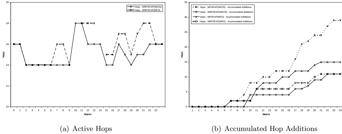
Figure 8.1: Used hops and accumulated hop additions for MPSFAP1 and MRPSFAP on NET2 for demand matrix series M_1 using MINLP Solver (NEOS) and MFD-R Heuristic
