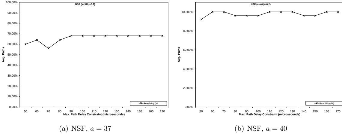
Figure 6.13: Feasibility Rate for NSF Network Topologies Using MFD Algorithm, as a Function of Delay Constraint
