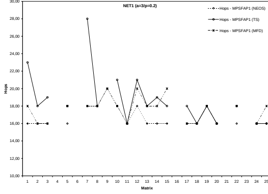
(a) Hops, a = 3
