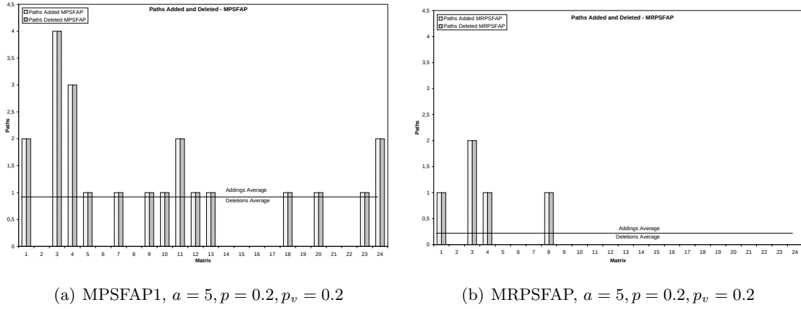
Figure 7.11: Path additions and deletions for MPSFAP1 and MRPSFAP for demand matrix series M_2
