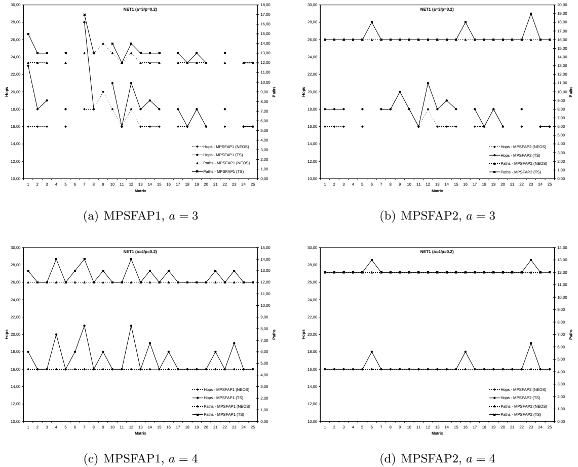
Figure 5.1: Results from MINLP Solver (NEOS) and Tabu Search (TS) for NET1
