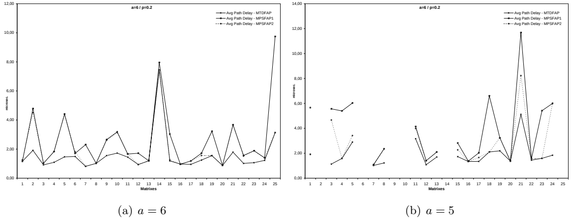
Figure 4.6: Average End-to-end Path Delay for NET2
