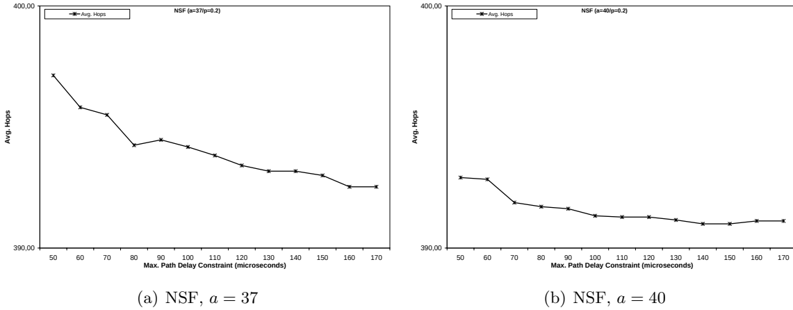
Figure 6.9: Average Quantity of Hops for NSF Network Topologies Using MFD Algorithm, as a Function of Delay Constraint
