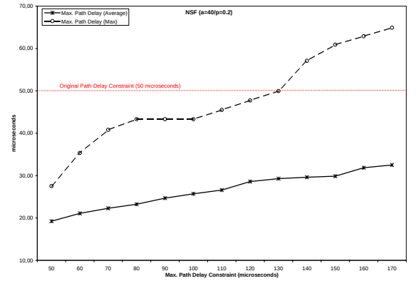
(b) NSF, a = 40
