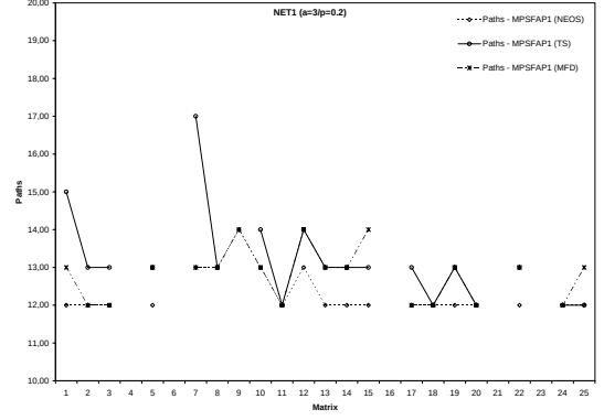
(b) Paths, a = 3
