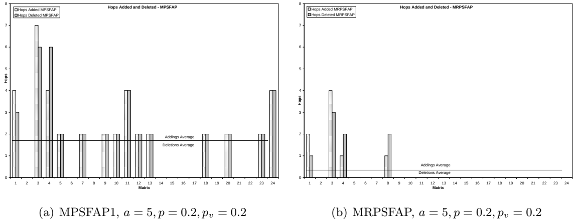
Figure 7.12: Hop additions and deletions for MPSFAP1 and MRPSFAP for demand matrix series M_2
