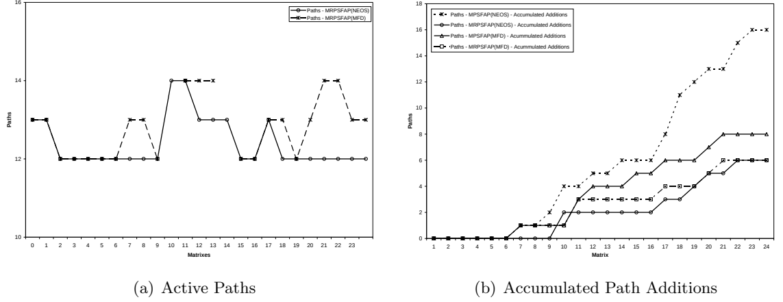
Figure 8.2: Used paths and accumulated path additions for MPSFAP1 and MRPSFAP on NET2 for demand matrix series M_1 using MINLP Solver (NEOS) and MFD-R Heuristic
