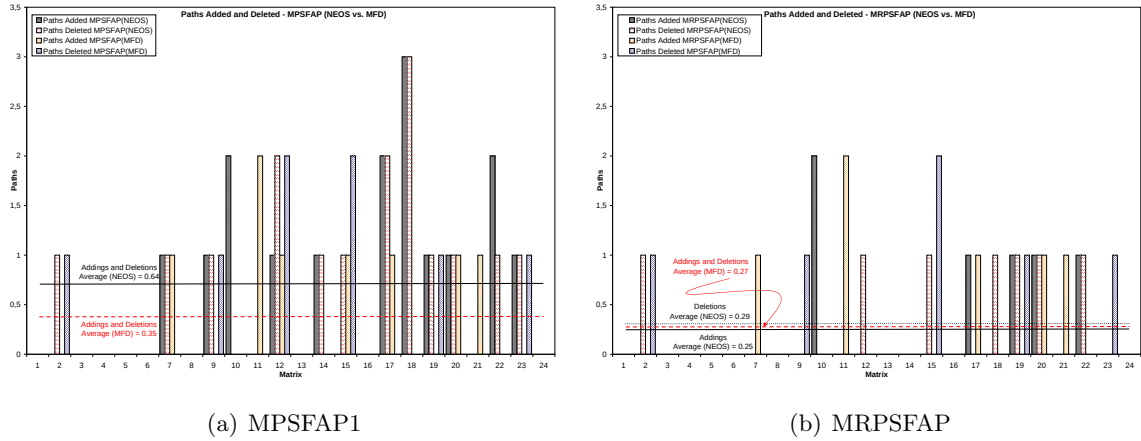
Figure 8.4: Paths added and deleted for MPSFAP1 and MRPSFAP on NET2 for demand matrix series M_1 using MINLP Solver (NEOS) and MFD-R Heuristic
