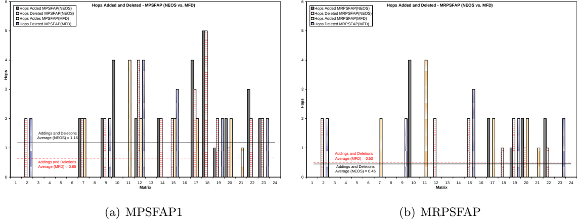
Figure 8.3: Hops added and deleted for MPSFAP1 and MRPSFAP on NET2 for demand matrix series M_1 using MINLP Solver (NEOS) and MFD-R Heuristic
