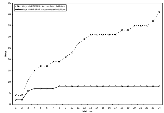
(b) Accumulated hops additions, a = 5, p = 0.2, p_v = 0.2
