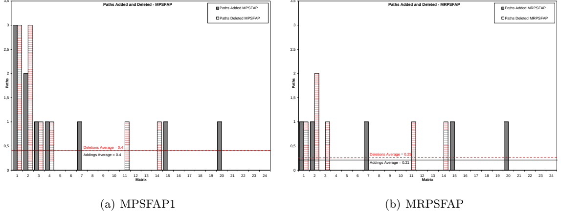
Figure 8.8: Paths added and deleted for MPSFAP1 and MRPSFAP on VTHD for demand matrix series M_1^{VTHD} using MINLP Solver (NEOS) and MFD-R heuristics
