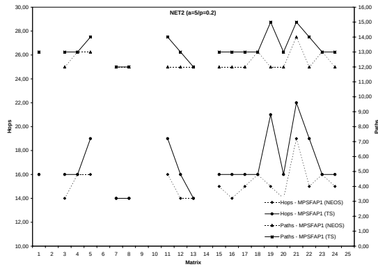
(a) MPSFAP1, a = 5
