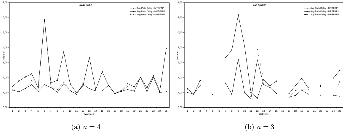
Figure 4.4: Average End-to-end Path Delay for NET1
