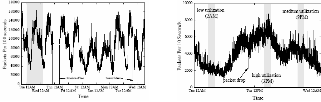
(a) Traffic per 100 seconds for 9 days packet trace (b) Traffic per 10 seconds for 27 hours packet trace
