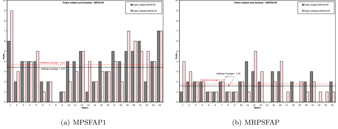
Figure 8.12: Paths added and deleted for MPSFAP1 and MRPSFAP on NSF for demand matrix series M_1^{NSF} using MINLP Solver (NEOS) and MFD-R heuristics
