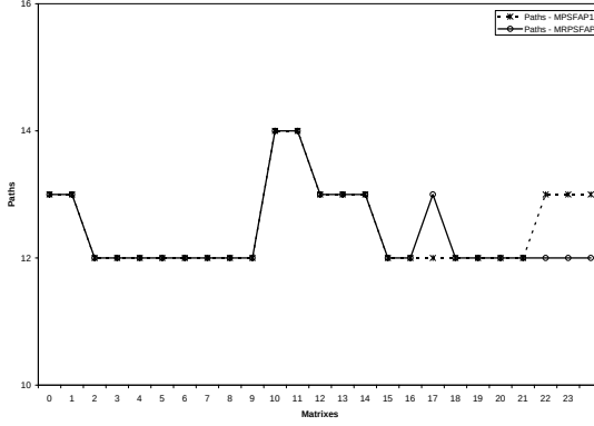
(a) Paths, a = 5, p = 0.2, p_v = 0.4
