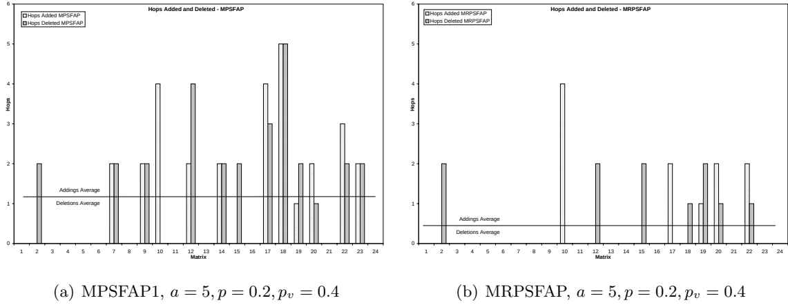
Figure 7.8: Hop additions and deletions for MPSPAF1 and MRPSFAP for demand matrix series M_1
