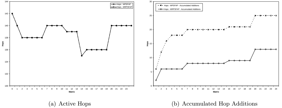
Figure 8.5: Active hops and accumulated hop additions for MPSFAP1 and MRPSFAP on VTHD for demand matrix series M_1^{VTHD} using MFD and MFD-R heuristics
