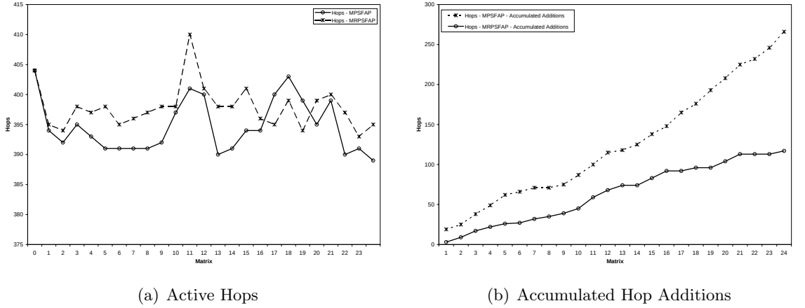
Figure 8.9: Active hops and accumulated hop additions for MPSFAP1 and MRPSFAP on NSF for demand matrix series M_1^{NSF} using MFD and MFD-R heuristics
