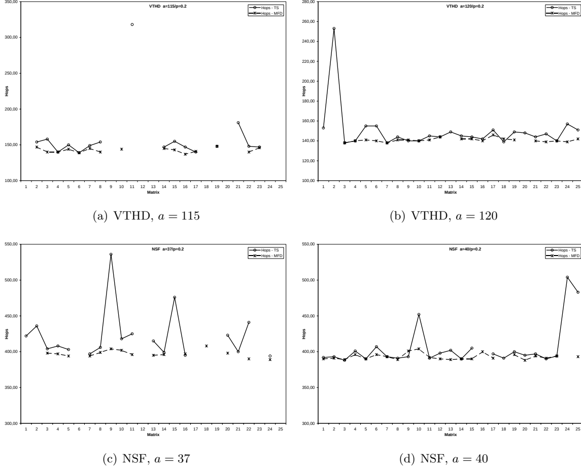
Figure 6.3: Value of The Objective Function for MPSFAP1 (Total Hops) for VTTHD and NSF Network Topologies using TS and MFD Algorithms
