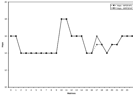
(a) Hops, a = 5, p = 0.2, p_v = 0.4
