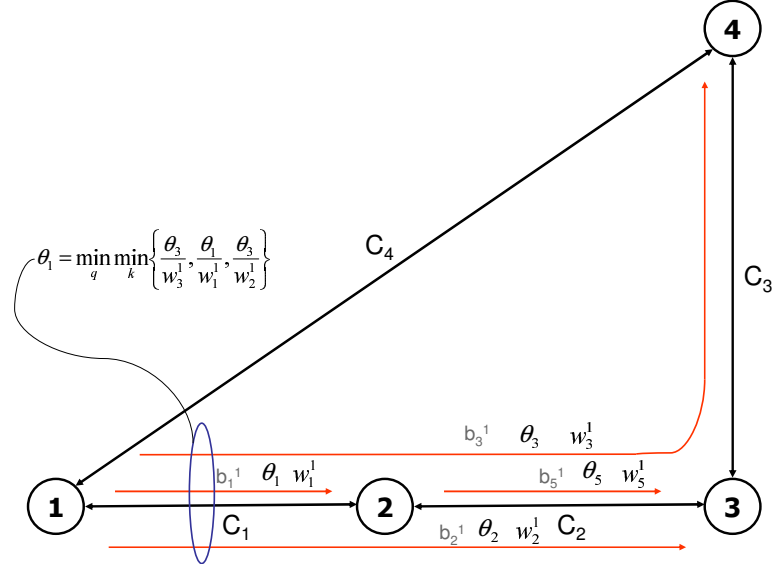
Figure 5.3: Modified Flow Deviation Algorithm: Path Delay Constraint Simplification
