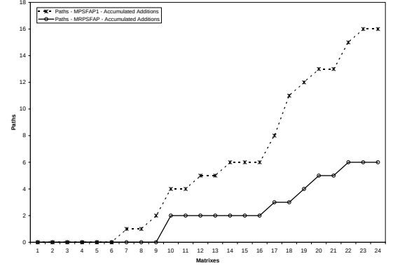
(b) Accumulated path additions, a = 5, p = 0.2, p_v = 0.4
