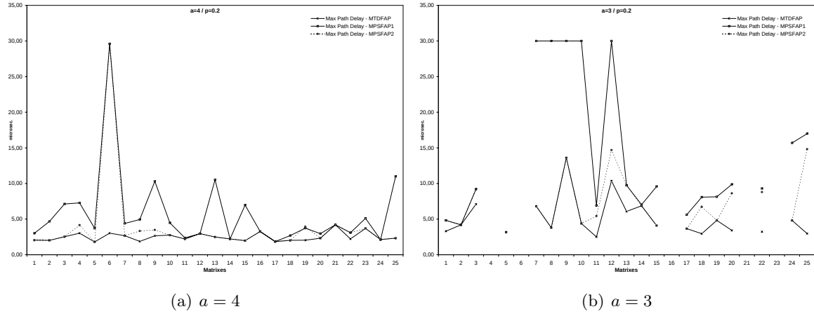
Figure 4.5: Maximum End-to-end Path Delay for NET1
