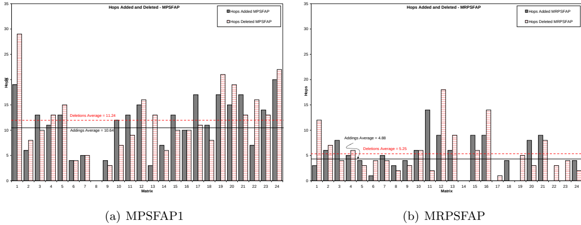
Figure 8.11: Hops added and deleted for MPSFAP1 and MRPSFAP on NSF for demand matrix series M_1^{NSF} using MINLP Solver (NEOS) and MFD-R heuristics
