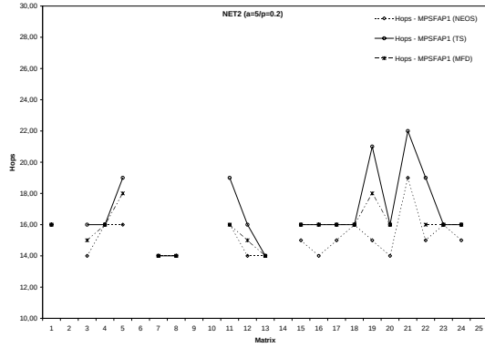
(a) Hops, a = 5
