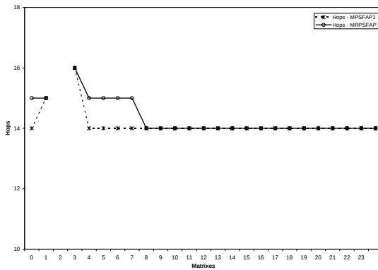
(a) Hops, a = 5, p = 0.2, p_v = 0.2
