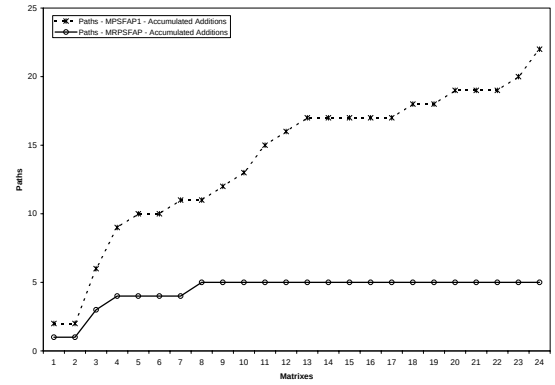
(b) Accumulated path additions, a = 5, p = 0.2, p_v = 0.2
