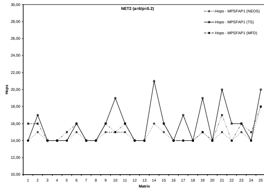
(c) Hops, a = 6
