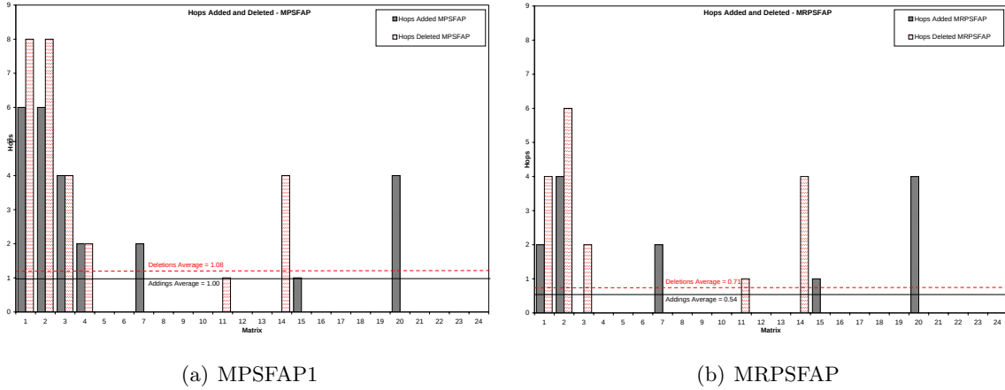
Figure 8.7: Hops added and deleted for MPSFAP1 and MRPSFAP on VTHD for demand matrix series M_1^{VTHD} using MINLP Solver (NEOS) and MFD-R heuristics
