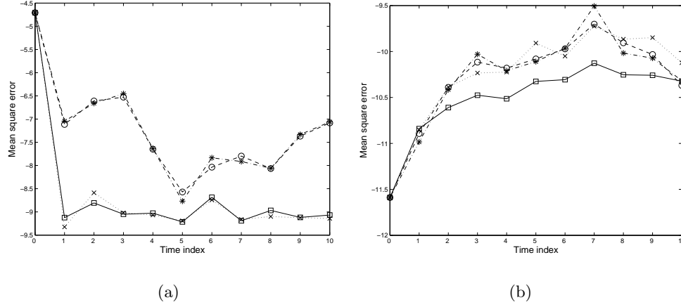
Fig. 4. Plot of MSE performances (on log-scale) of the bootstrap particle filter (*), the SSAPF based on optimal weights (□), the SSAPF based on the generic weights t_k^{P\&S} (○), and the fully adapted SSAPF (×) for the ARCH model in Section 5.1. The MSE values are computed using 10,000 particles and 400 runs of each algorithm.
