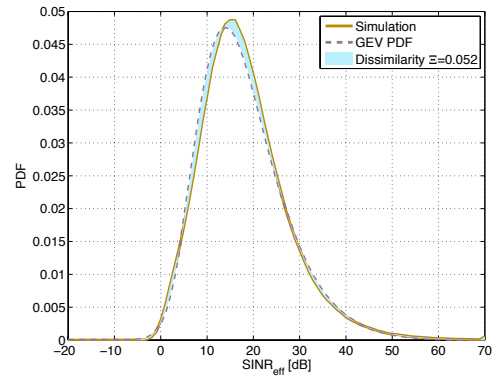
Fig. 3. SINR_{eff} distribution through simulation and GEV polynomial for \sigma_{SH} = 9 dB, R = 1500 m, P_{Tx} = 43 dBm and reuse 3x3x3.
