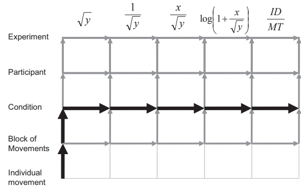
Figure 3. The statistical-aggregation and calculation steps involved in the computation of a TP_M . One example path is highlighted, which delivers the TP_M value of one particular participant for one particular condition.
